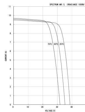
Fig. 4 I-V characteristics of KK280P-3CD3CG at various cell temperatures.
