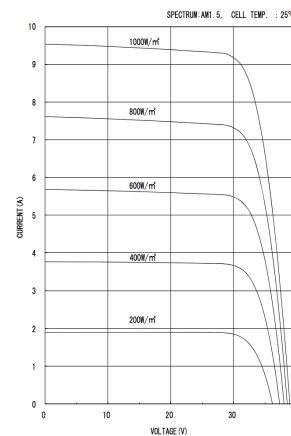
Fig. 5 I-V Characteristics of KK280P-3CD3CG at various irradiance levels.
